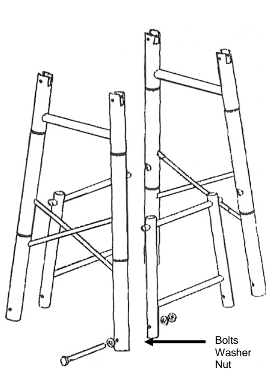
Figure 7 Place the Leg Supports (#12) between the Legs so that the post on the support faces the hole on a corresponding leg. Attach Bolts at the bottom of each leg.
